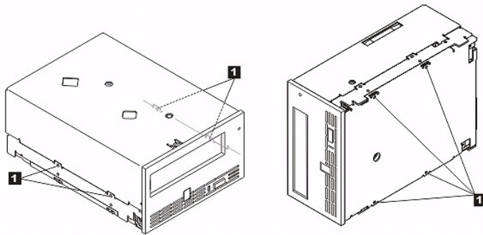
Figure 8. Mounting Holes on Tape Drive
