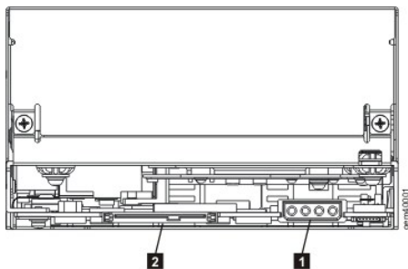
Figure 4. Rear Panel of Internal SAS Tape Drive
